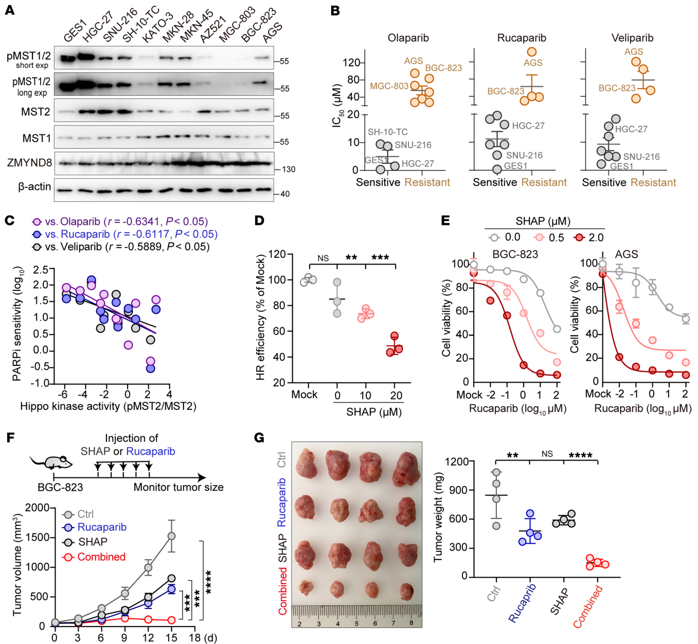
Figure 8. Rational restoration of Hippo kinase activity resensitizes tumors to PARP inhibition. (A) Western blot analysis of p-MST1/2 and ZMYND8 across 11 GC cell lines. (B) IC_{50} values measured from the GC cell lines after they were treated with each PARPi. A group was defined to be sensitive or resistant to PARPi based on whether the IC_{50} was, respectively, less than or greater than 20 \mu M . (C) Linear regression analysis of PARPi sensitivity and Hippo kinase activity across the GC cells. (D) Plot showing a dose-dependent suppression of HR repair by SHAP ( n = 3 ). (E) Plots showing that treatment of GC cells with SHAP resensitized the cells to PARPi. Specifically, BGC-823 and AGS cells were each treated with various doses of rucaparib in the presence of 0, 0.5, and 2.0 \mu M SHAP for 24 hours. (F and G) Results showing that SHAP treatment dramatically enhanced rucaparib-mediated antitumor efficiency in vivo. Nude mice bearing GC tumors were intraperitoneally administered SHAP and rucaparib, either alone or in combination. (F) Tumor size was measured every 3 days, and (G) tumors were photographed and weighed on day 18 ( n = 4 mice/group). **P < 0.01 , ***P < 0.001 , and ****P < 0.0001 , by 1-way ANOVA with Dunnett's post hoc test (D and G) and unpaired Student's t test (F). See also Supplemental Figure 9.
